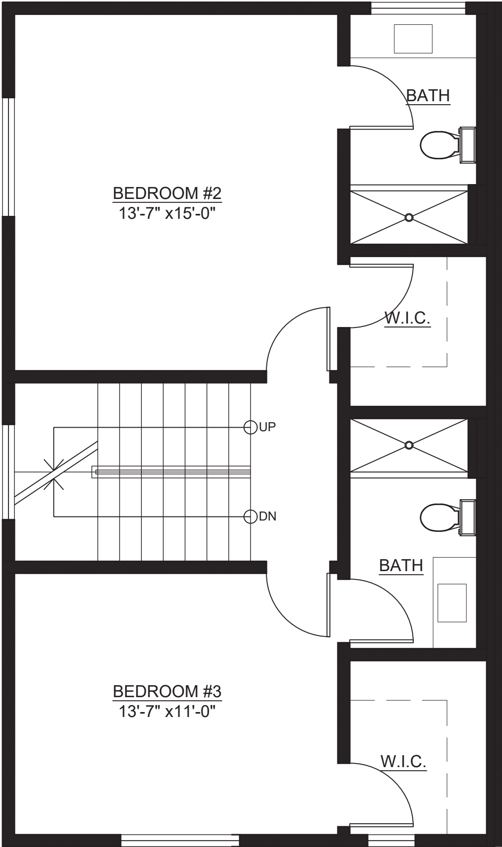
LAYOUT 1: 3RD FLOOR
