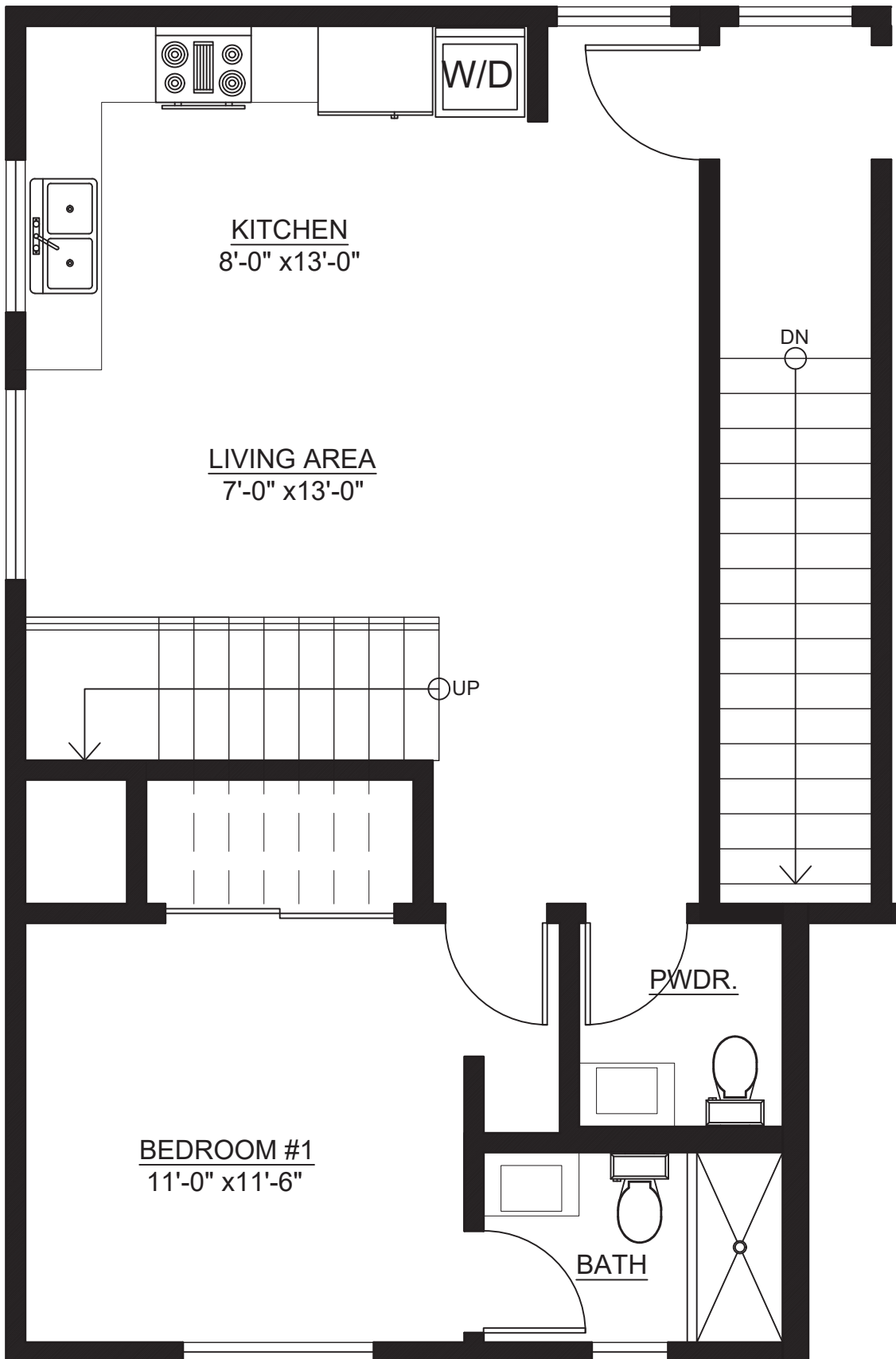
LAYOUT 1: 2ND FLOOR
